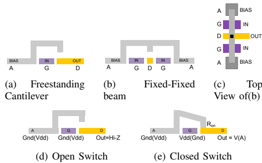
Fig. 1. (a)-(c) NEMS-CNT Device Structures; (d)-(e) Voltage biases on terminals for different logic states
