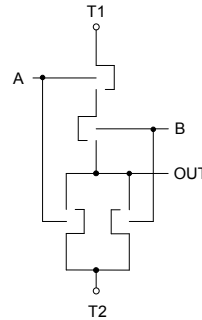
(a) NAND/NOR circuit with Standard design technique (4 cantilevers). Each NEMS device corresponds to a MOSFET device in a CMOS-based NAND circuit.
