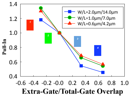
(a) Normalized Pull-in Voltage
