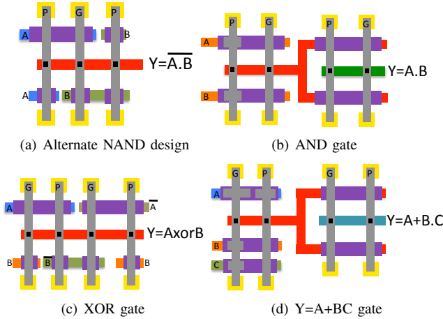
Fig. 5. NEMS-WAL designs of adder components
