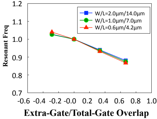
(b) Normalized Resonant Frequency
