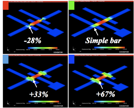
Fig. 2. Weighted gate overlap structures simulated
