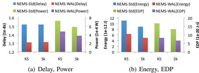
Fig. 6. Comparing Std and WAL designs for 32-bit adders
