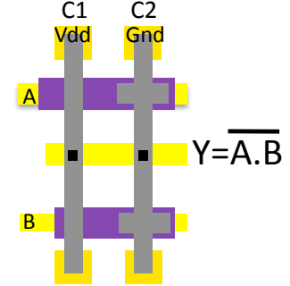
(b) NAND/NOR circuit with NEMS-WAL design (2 cantilevers) - Top view. Cantilevers C_1 and C_2 have a weighted overlap area with gates A and B.
